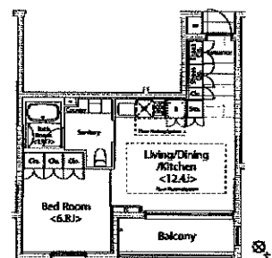
■ O-type 1LDK/ 44.35㎡[13.41#]
