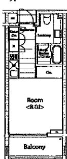
■ J1-type 1K / 27.26㎡(8.24坪)
