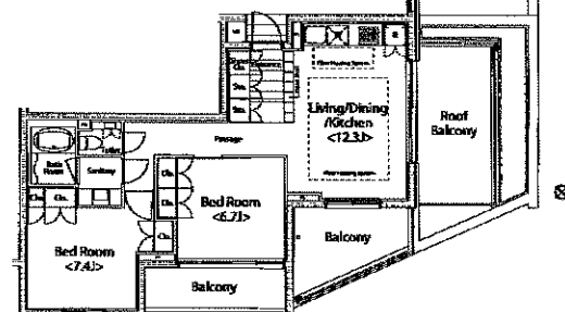
■ U-type 2LDK+RoofBalcony/ 64.79㎡[19.57#]
