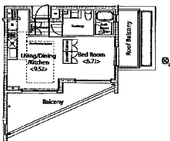
■ S-type 1R+RoofBalcony/ 36.51㎡[11.04#]
